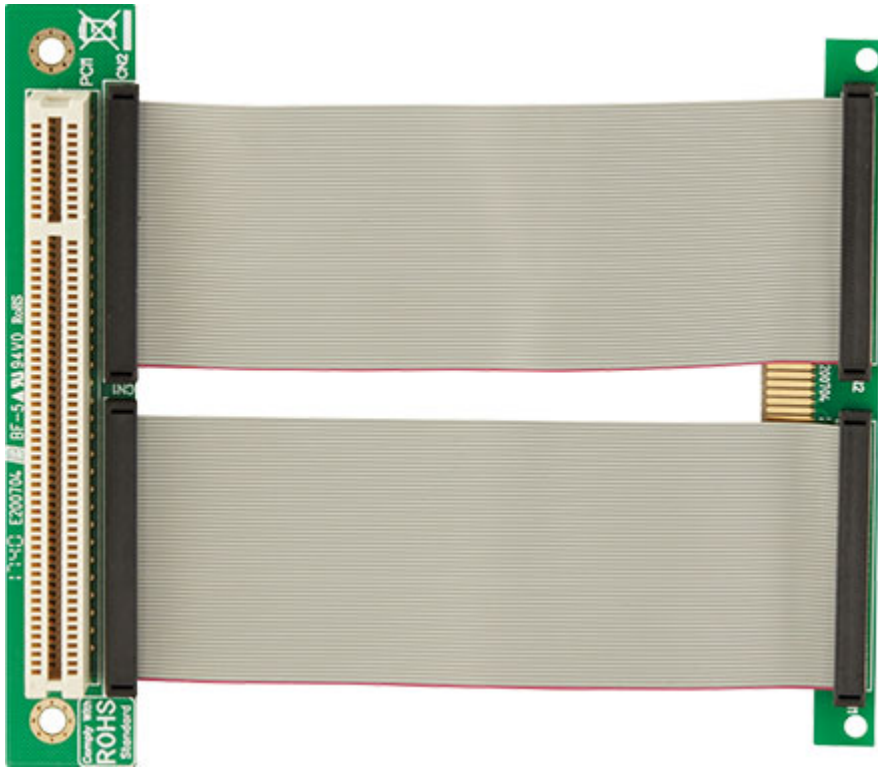
PCI to PCI riser card, L=100 mm
